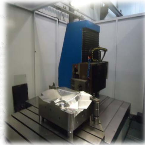
CNC DRILLING MACHINE Max. Dimensions: X (1000) Y (600) Z (600)
