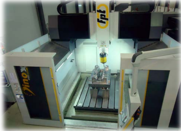
5 AXIS FPT CNC MILLING MACHINE Max. Dimensions: X (2500) Y (2200) Z (1100)
